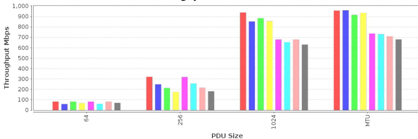
Throughput vs PDU Size
